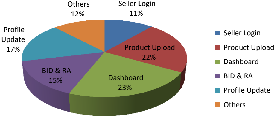
Issue Count
